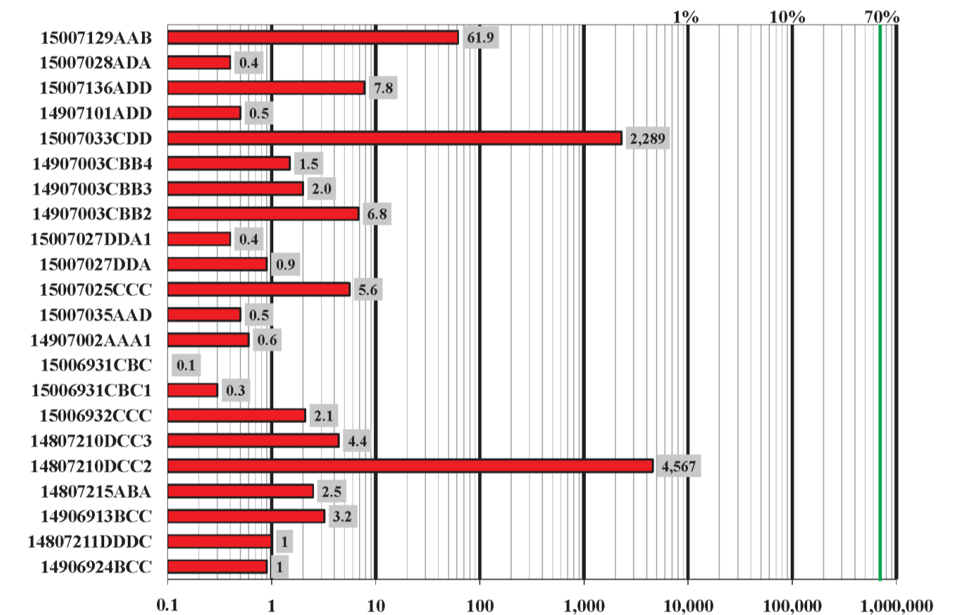
Figure 1. Graph depicting the relative relationship and absolute maximum values of flame-ionization detector (FID) instrument responses from selected wells in Wells County. FID results for each well are presented in order of field screening occurrence from top to bottom. Values shown are those reported from the ground-water/air interface (GWI) (as CH 4 in ppm). The concentration of methane typical in commercial natural gas is highlighted by the vertical green line at 70%.
