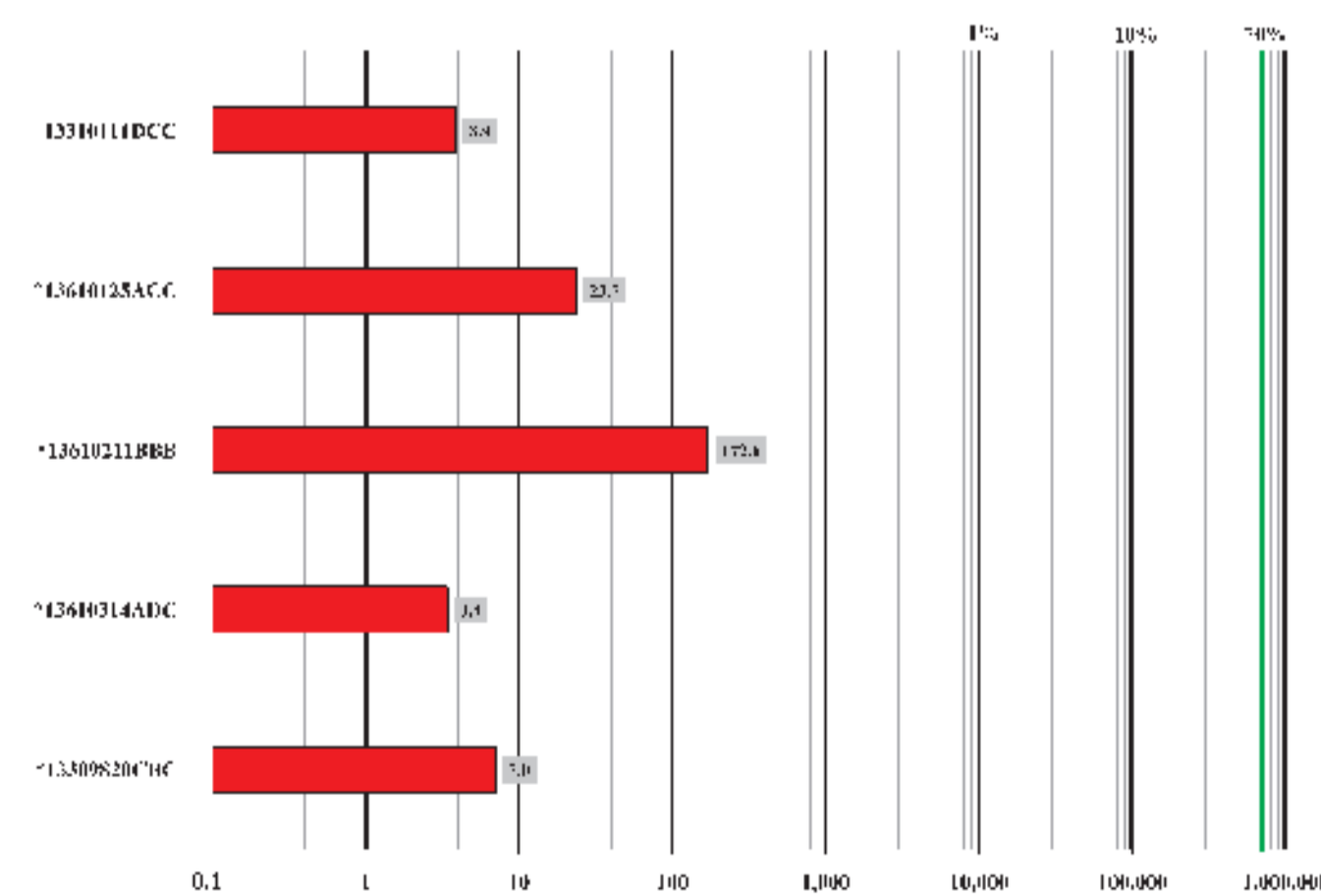
Figure 1. Graph depicting the relative relationship and absolute maximum values of flame-ionization detector (FID) instrument responses from selected wells in Slope County. FID results for each well are presented in order of field screening occurrence from top to bottom. Values shown are those reported from the ground-water/air interface (GWI) (as CH 4 in ppm). The concentration of methane typical in commercial natural gas is highlighted by the vertical green line at 70%.
